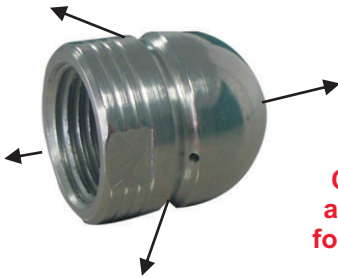
1 forward, 3 back ports
